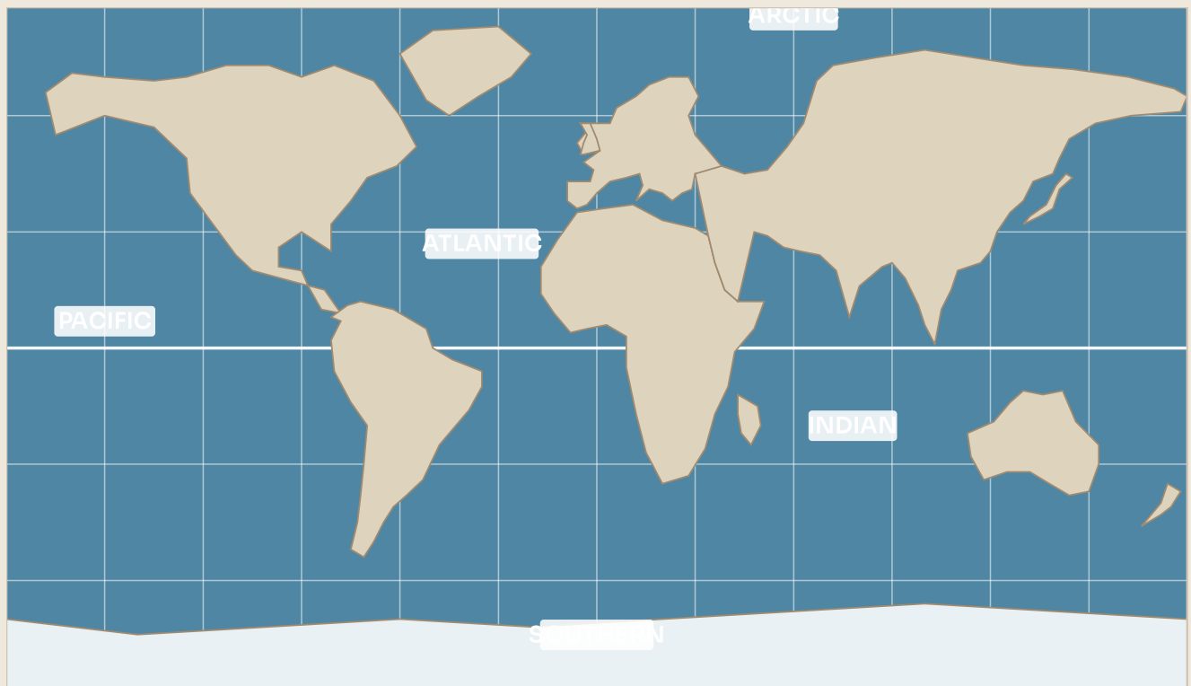
Figure 4.2 • The five oceans.
