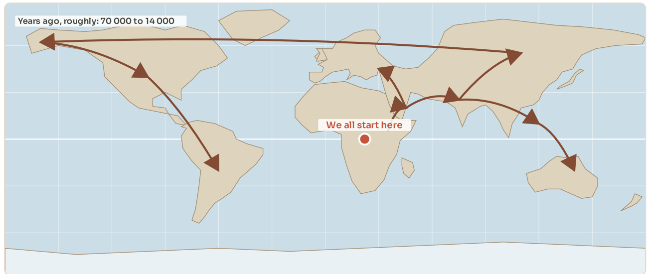
Figure 6.1 • Out of Africa.
