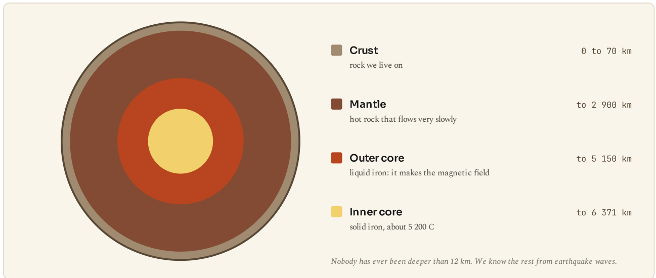
Figure 3.1 • Inside the Earth.
